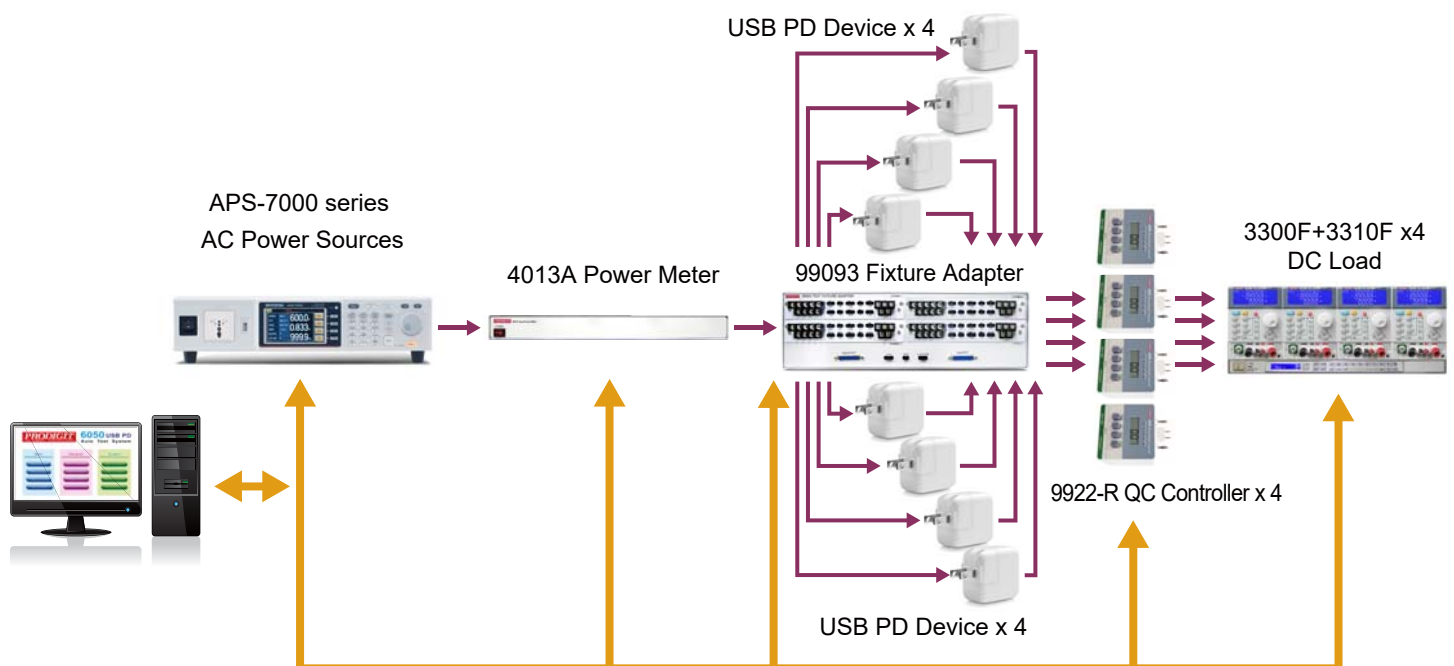
6050-4-A-X 4 Channel with AB Switch Test System Configuration
