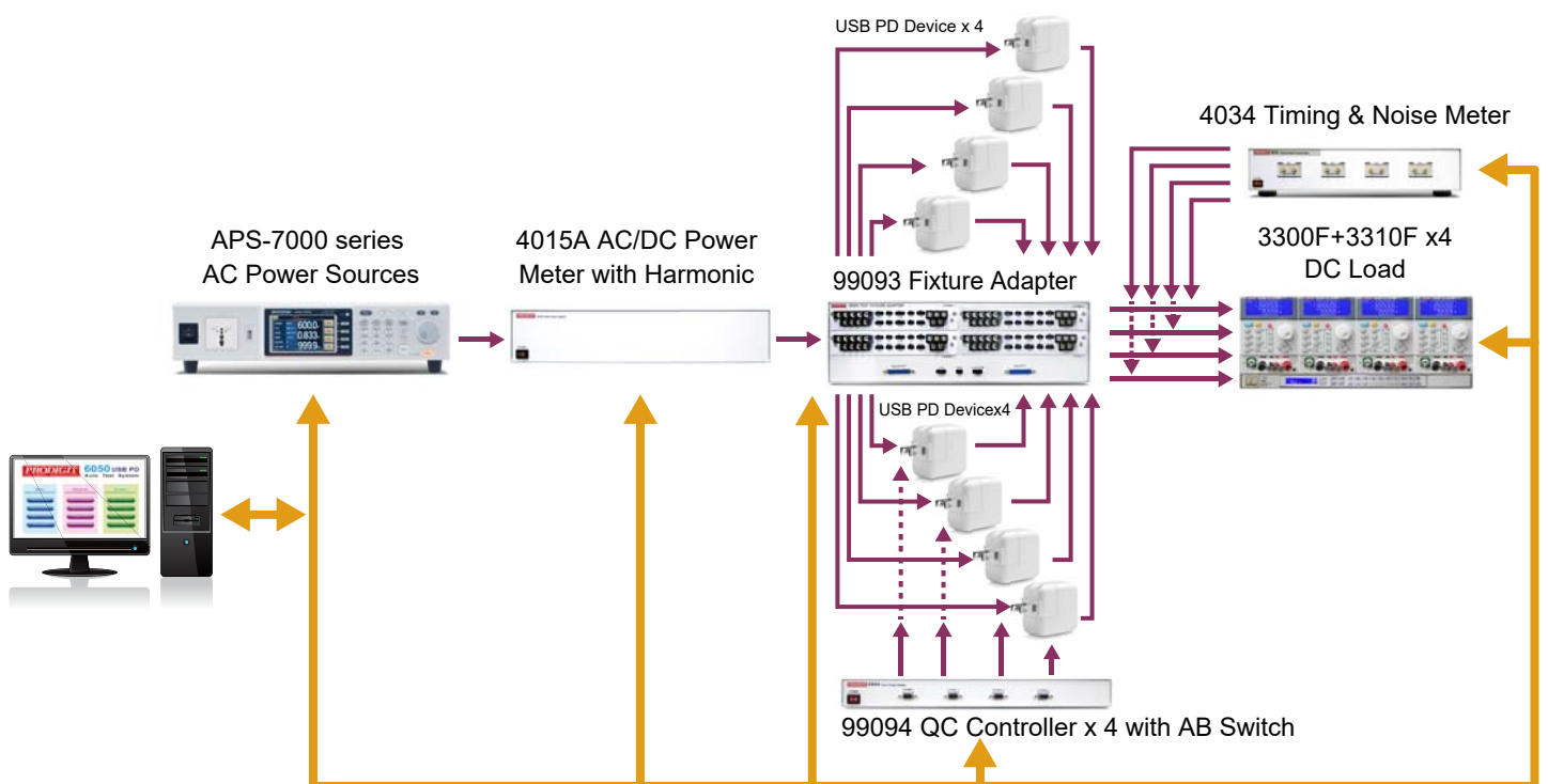
6050-4-C-X 4 Channel with AB Switch Test System Configuration
