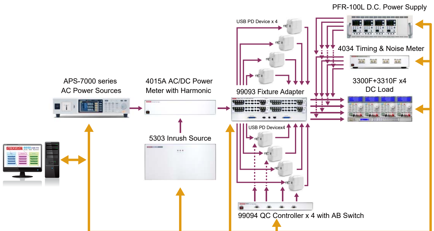
6050-4-D-X 4 Channel with AB Switch Test System Configuration
