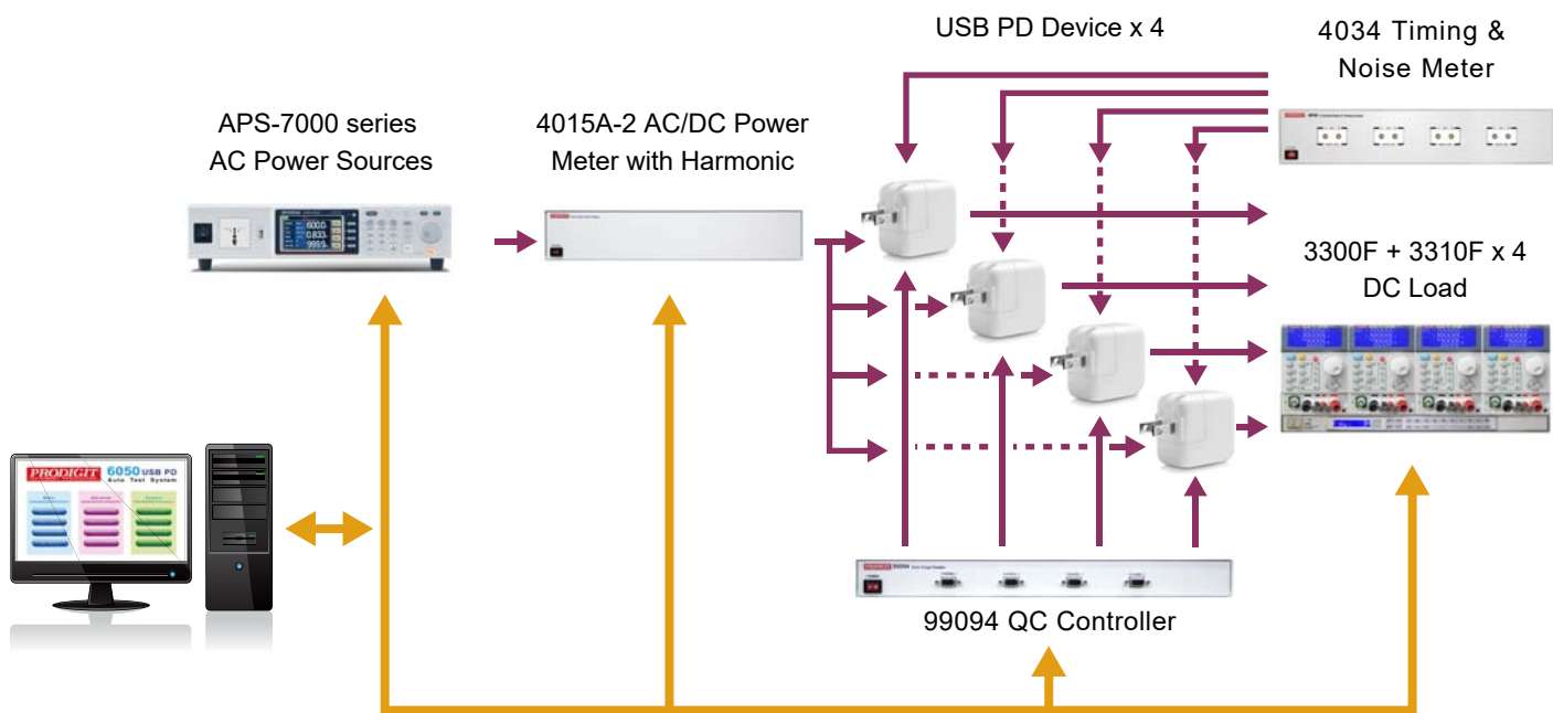
6050-4-C 4 Channel Test System Configuration
